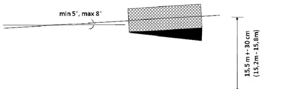
Diagram 3.1b: Ramp Angle
