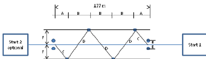
Diagram 6.3: Slalom short
