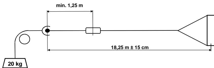
Diagram 2.4: Tow lines made with Spectra ropes
