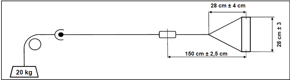
Diagram A1.5: Handle Dimensions in Jump and Slalom
