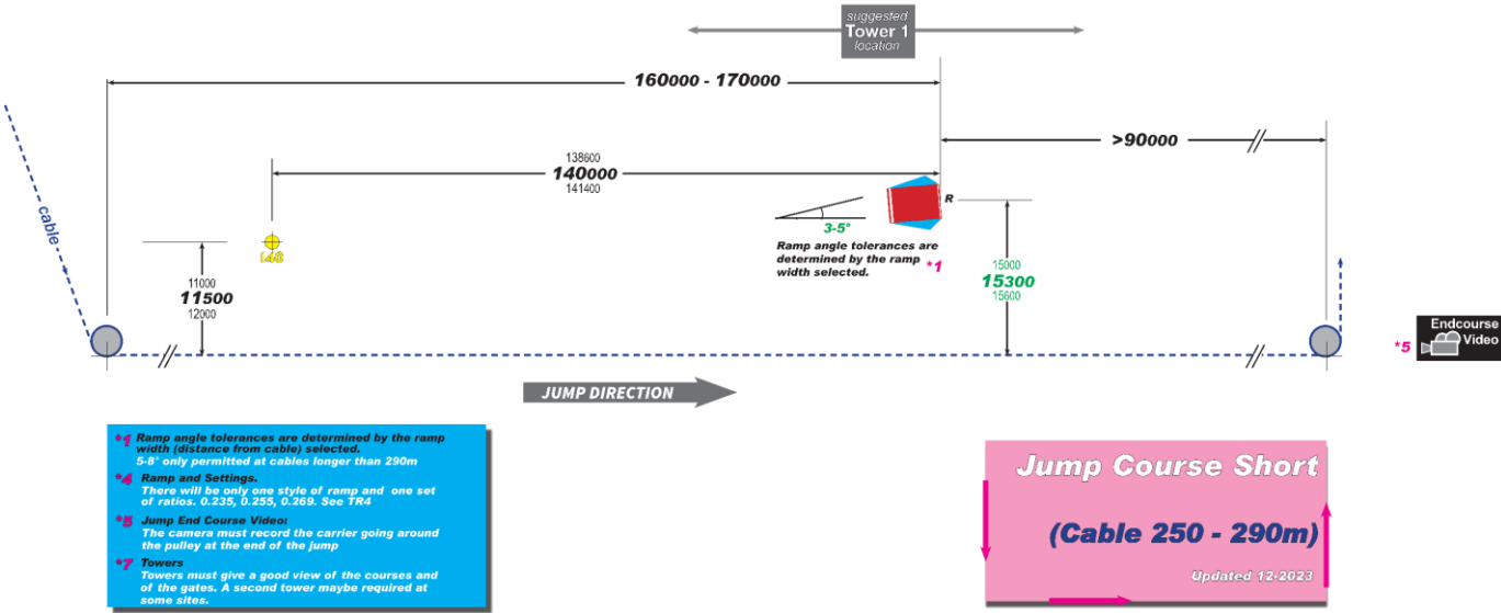
Diagram A2.2: Jump Course (short > 250m)
