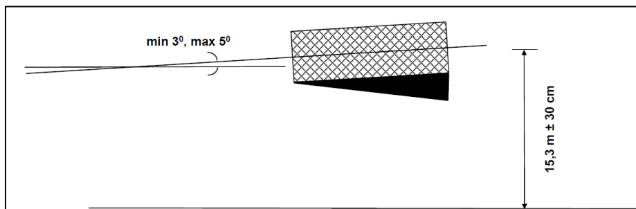
Diagram A2.1a: Ramp angle small angle (3 - 5° open)
