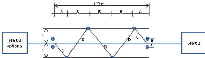
Diagram 6.3: Slalom short
