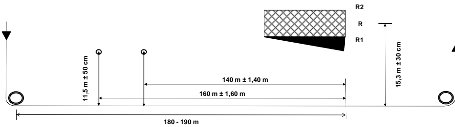
Diagram 3.2: Jump Course (long > 300m)
