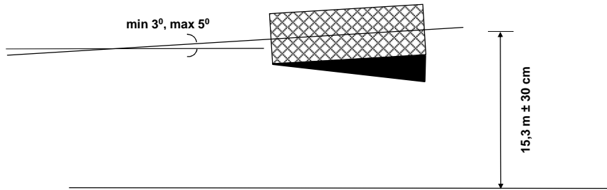
Diagram 3.1: Ramp Angle
