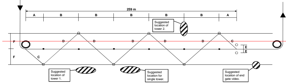
Diagram 4.1: Slalom Course
