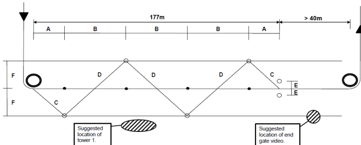
Diagram 4.3: S4 Slalom Course (short > 220m)
