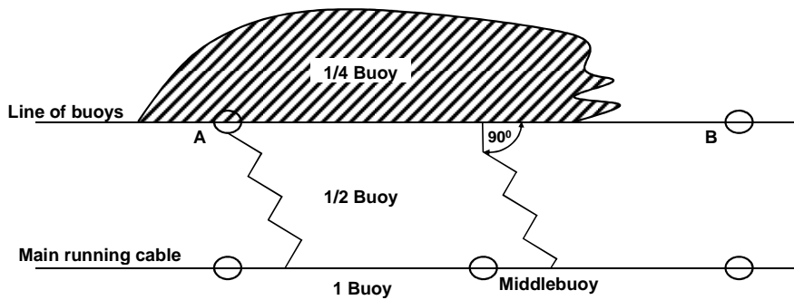
Diagram 4.1.2: Scoring of buoys
